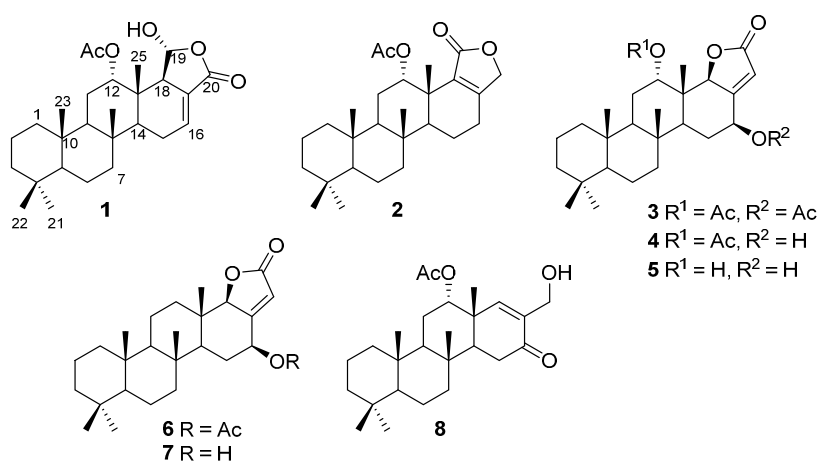
Figure 1. Structures of the isolated scalarane sesterterpenoids.
